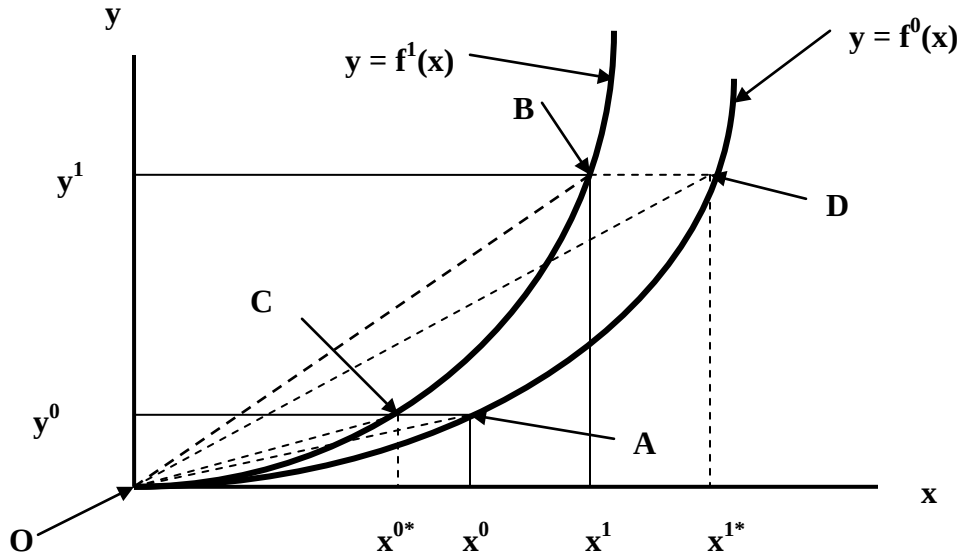
Figure 1: Returns to Scale Measures in the One Output, One Input Case
