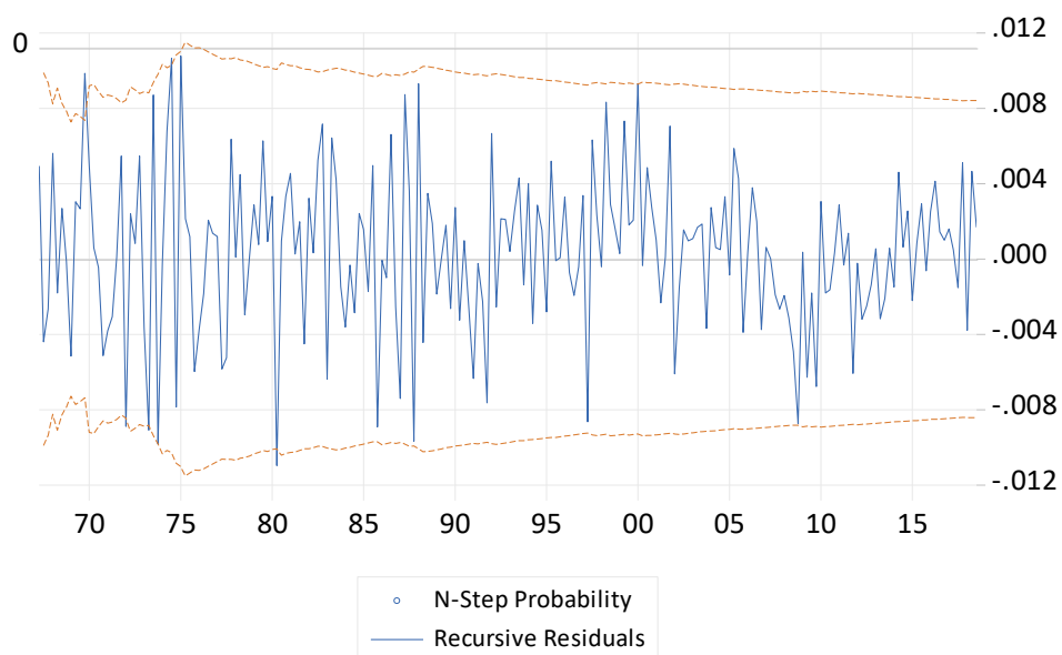
Recursive Least Squares N-Step Forecast Test: 1964Q4-2018Q3
