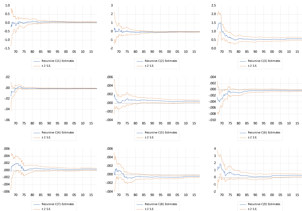
Recursive Least Squares Coefficient Plots: 1964Q4-2018Q3
