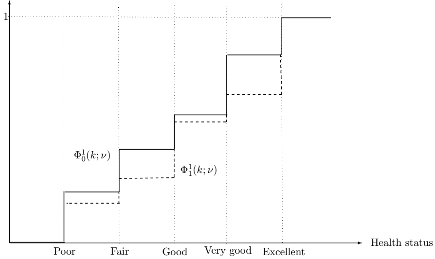
Figure 1: Theorem 1
