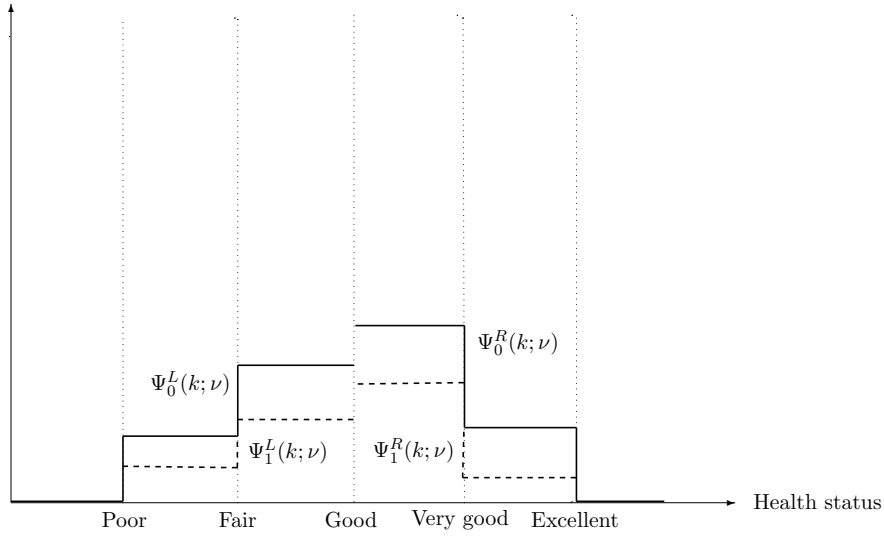
Figure 2: Theorem 4
