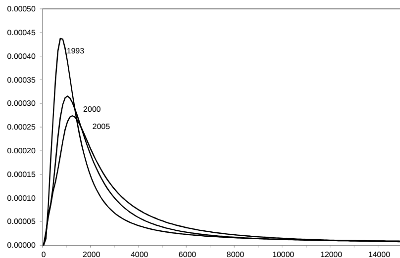
Figure 3: Global Density Function over Time (using ICP PPP data in constant 2005 prices)
