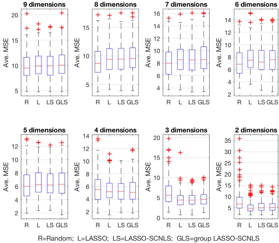
Figure B1. Results with 200 replications for DGP 2
