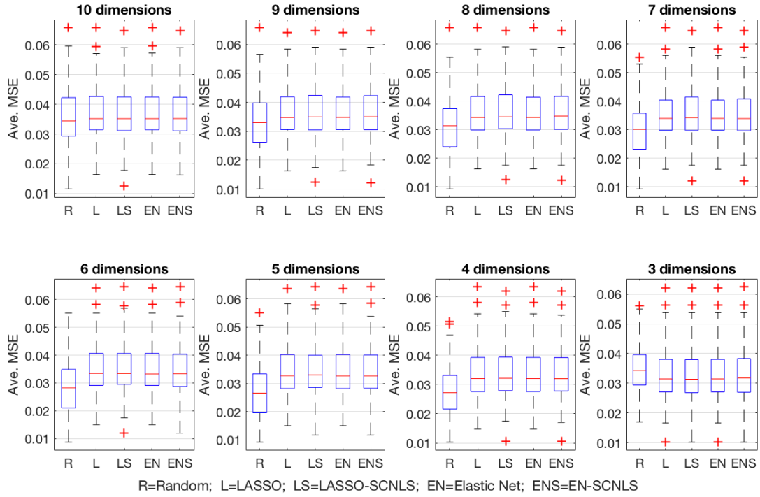
Figure B5. AMSE with 200 replications for Case C
